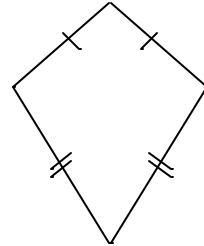
kite
