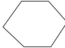
hexagon
