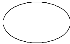
ellipse
