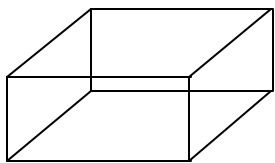
rectangular prism
