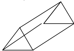
triangular prism
